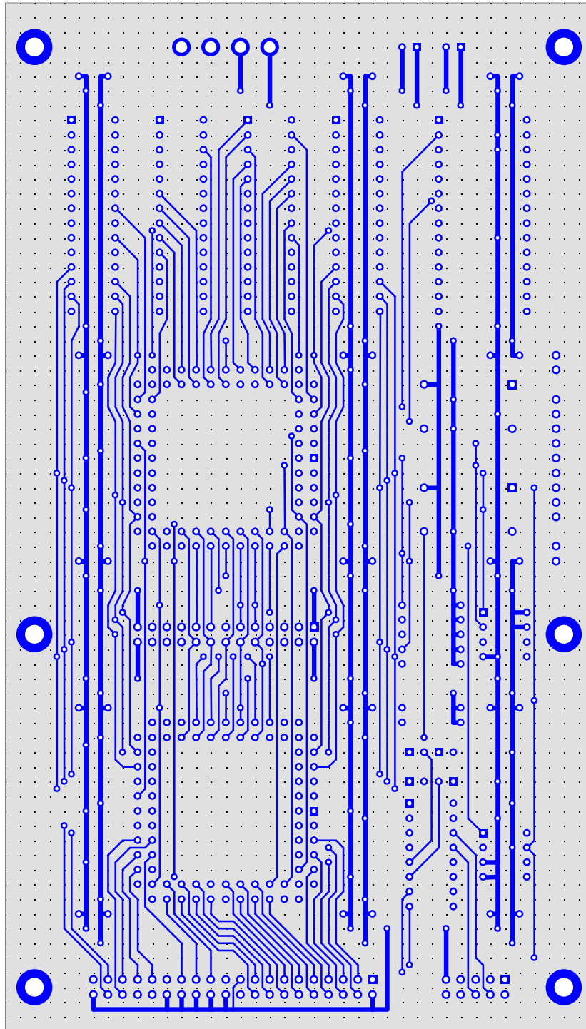
C:\WINNT\Profiles\dconroy\Desktop\pdp8x_16.pcb (Bottom layer)
