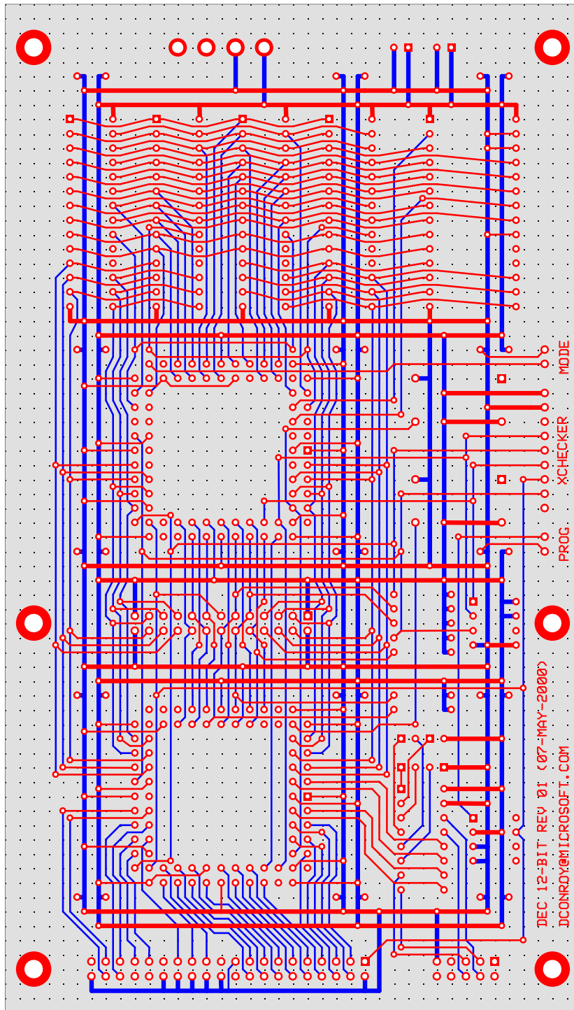
C:\WINNT\Profiles\lconroy\Desktop\pdp8x_16.pcb (Top layer, Bottom layer)
